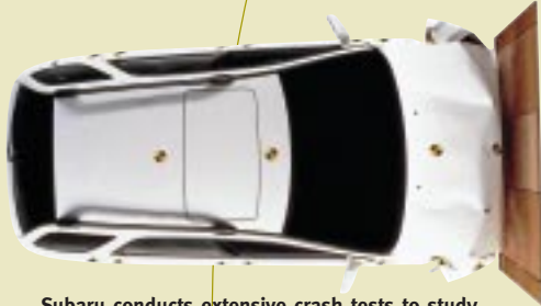
Subaru conducts extensive crash tests to study how vehicles perform under extreme conditions.
